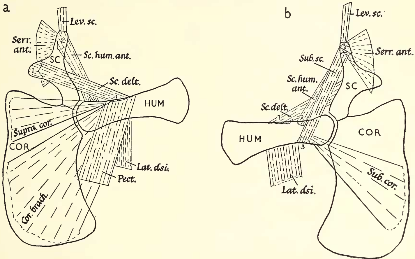
TEXT-FIG. 4. Diagrammatic reconstruction of pectoral girdle of Stretham Pliosaur. \times \frac{1}{16} . a , Ventral view; b , Dorsal view. COR., Coracoid; HUM., Humerus; sc., Scapula. Muscles: cor. brach. , coracobrachialia; lat. dsi. , latissimus dorsi; lev. sc. , levator scapulae; pect. , pectoralis; sc. delt. (1), scapular deltoid; sc. hum. ant. (2), scapulo-humeralis anterior; serr. ant. , serratus anterior; sub. cor. , subcoracoideus; sub. sc. (3), subscapularis; supra. cor. , supracoracoideus. Nos. 1, 2, 3 indicate insertions or origins.
